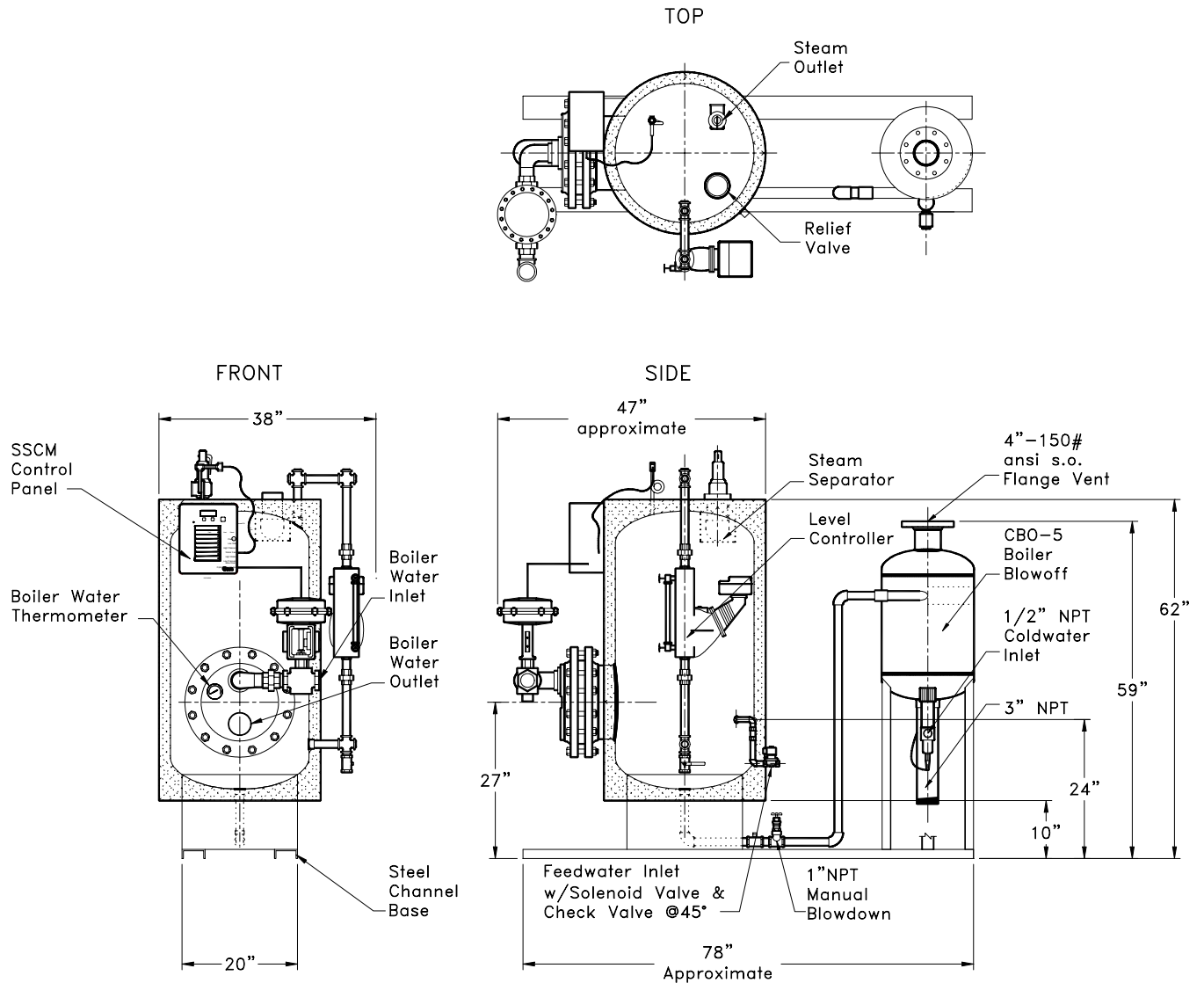
V90USG-W-CBO Energy Source-Boiler Water
