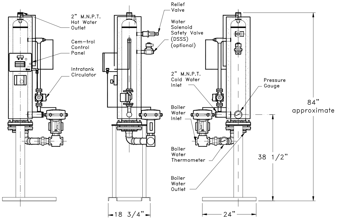
V6SEH636 Energy source – boiler water
