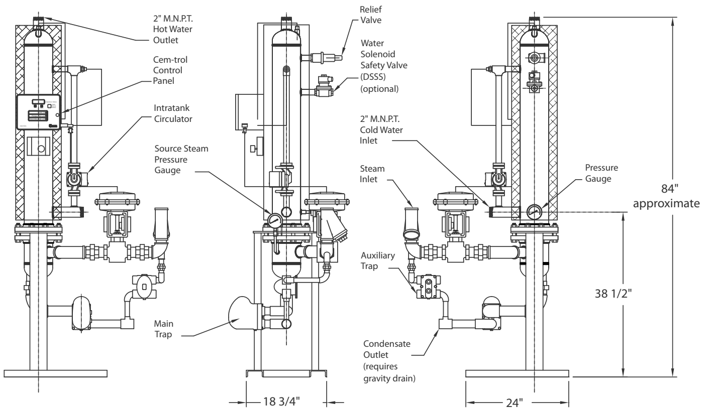
V6SEH624 Energy source - Steam
