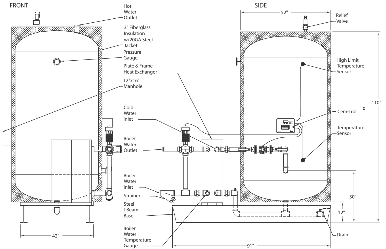
V680SPH-PF-3W PLATE & FRAME HEAT EXCHANGER
