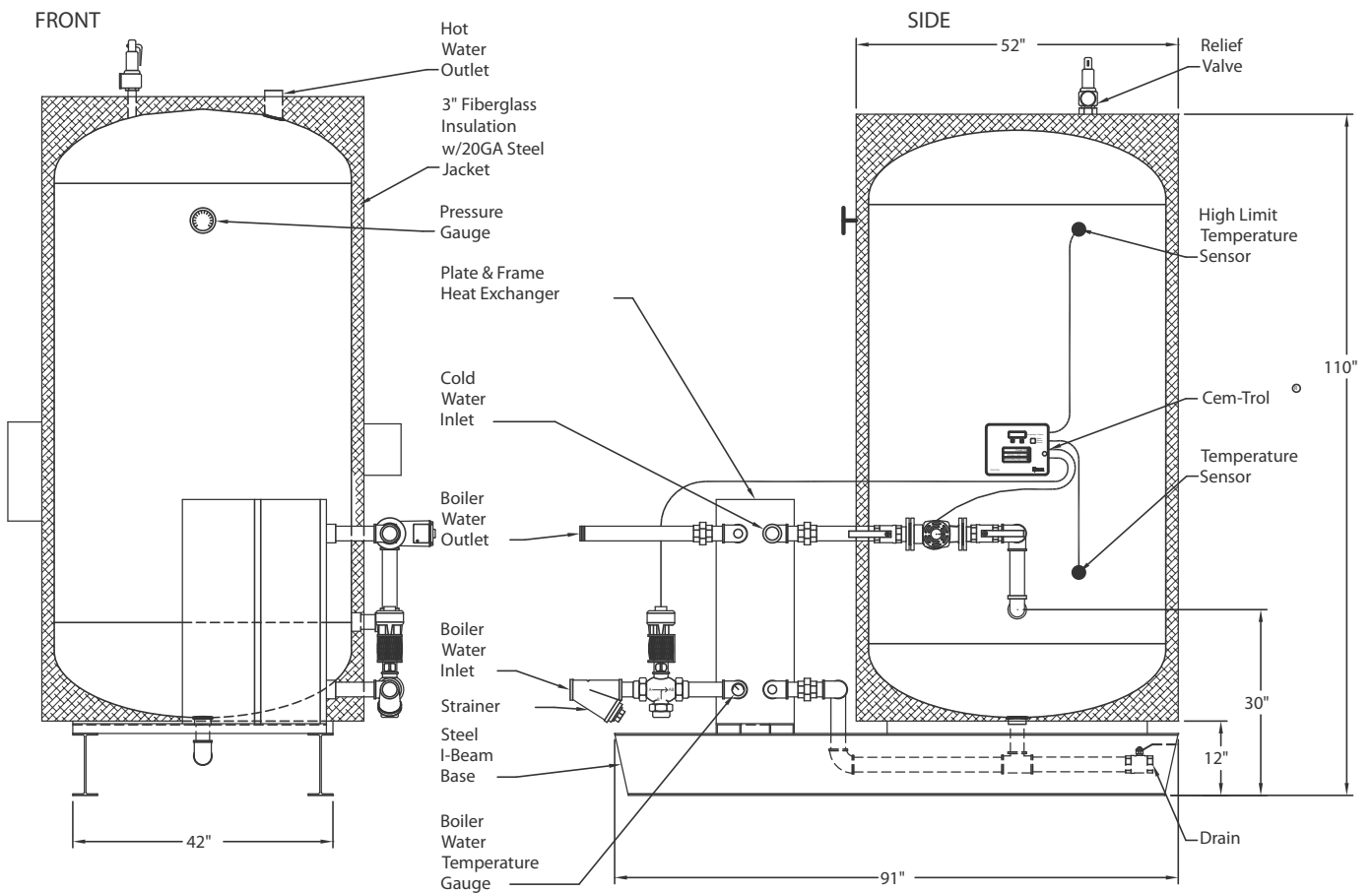
V680SPH-PF-2W PLATE & FRAME HEAT EXCHANGER
