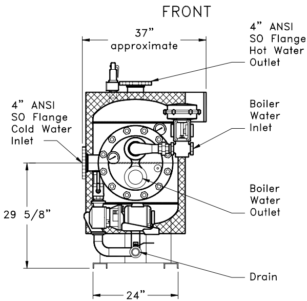
V60SSH14XX-W Energy Source - Boiler Water
