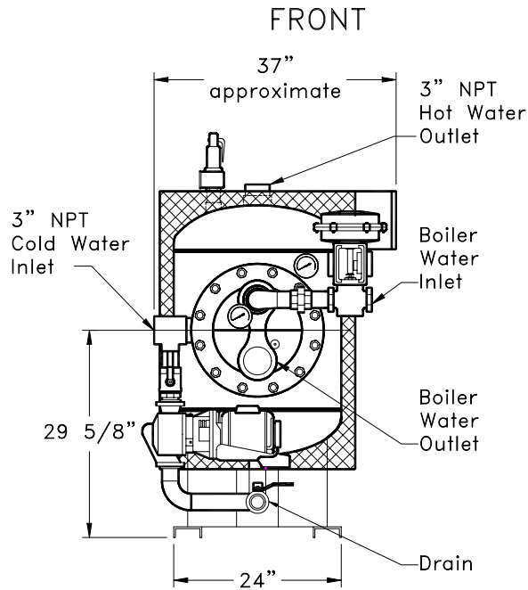
V60SSH12XX-W Energy Source-Boiler Water
