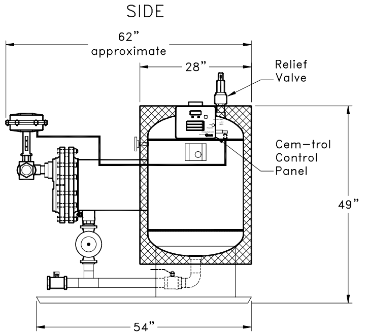
V60SSH12XX-W Energy Source-Boiler Water
