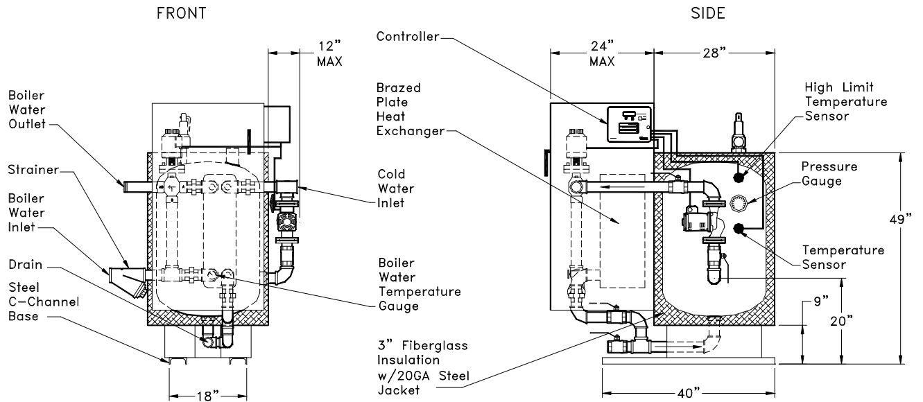
V60SPH-BP-3W BRAZED PLATE HEAT EXCHANGER
