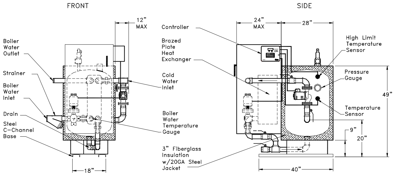
V60SPH-BP-2W BRAZED PLATE HEAT EXCHANGER
