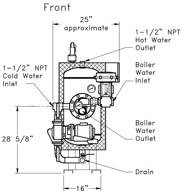
V30SSH6XX-W Energy Source - Boiler Water
