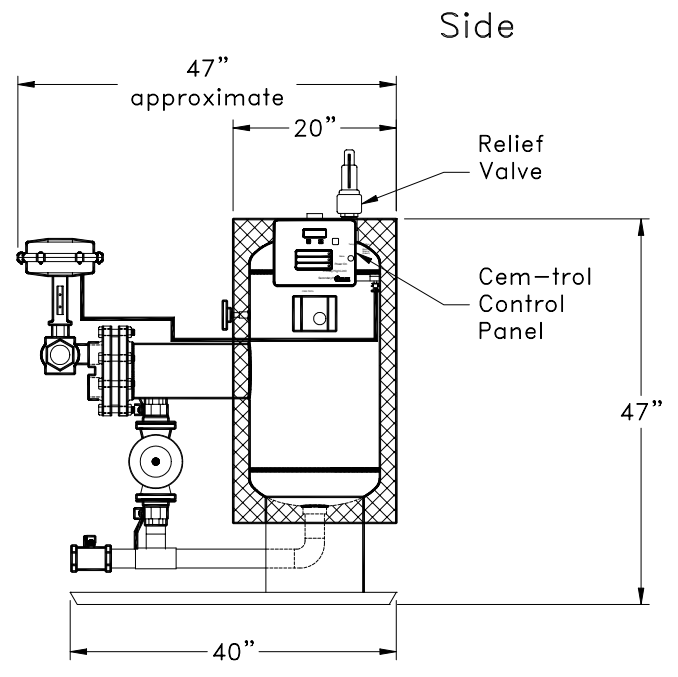
V30SSH6XX-W Energy Source - Boiler Water
