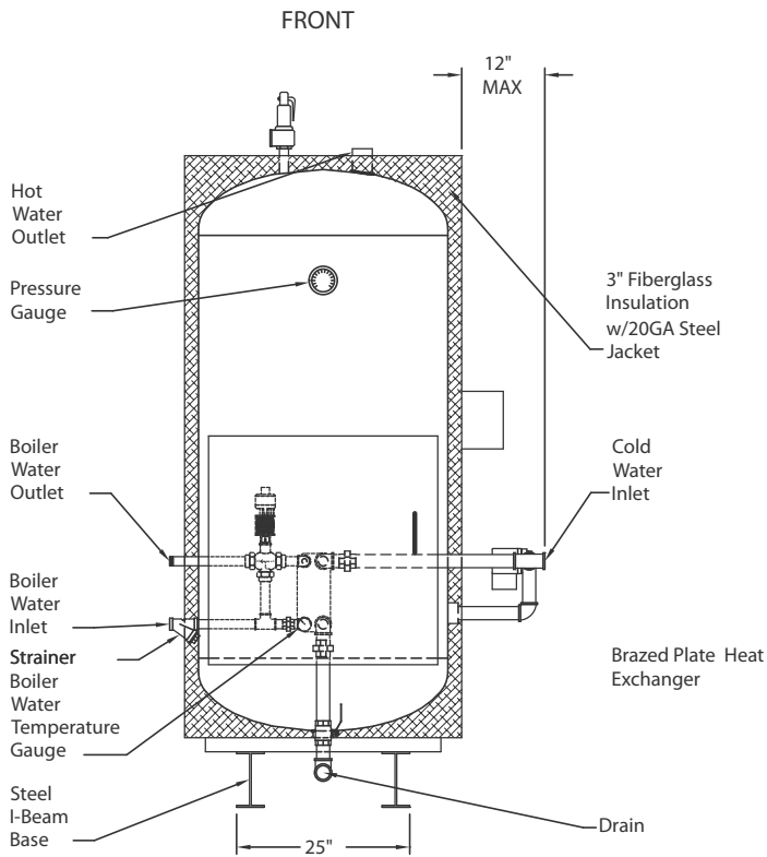
V300SPH-BP-3W BRAZED PLATE HEAT EXCHANGER
