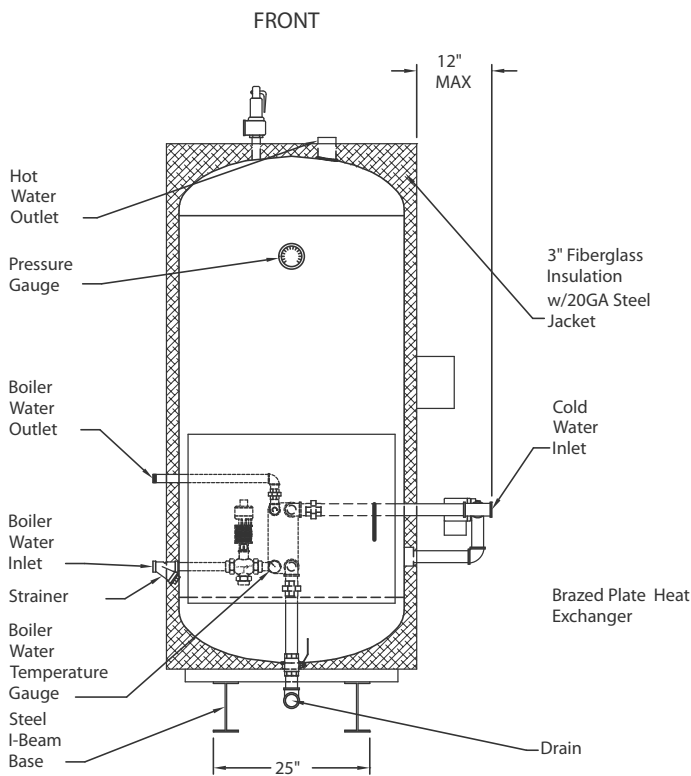
V300SPH-BP-2W BRAZED PLATE HEAT EXCHANGER
