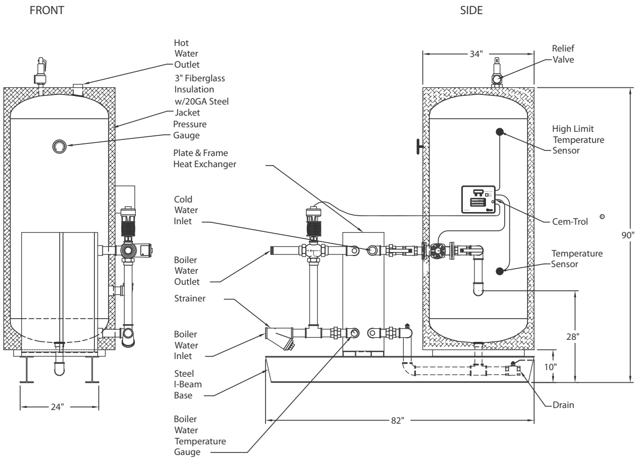
V200SPH-PF-3W PLATE & FRAME HEAT EXCHANGER
