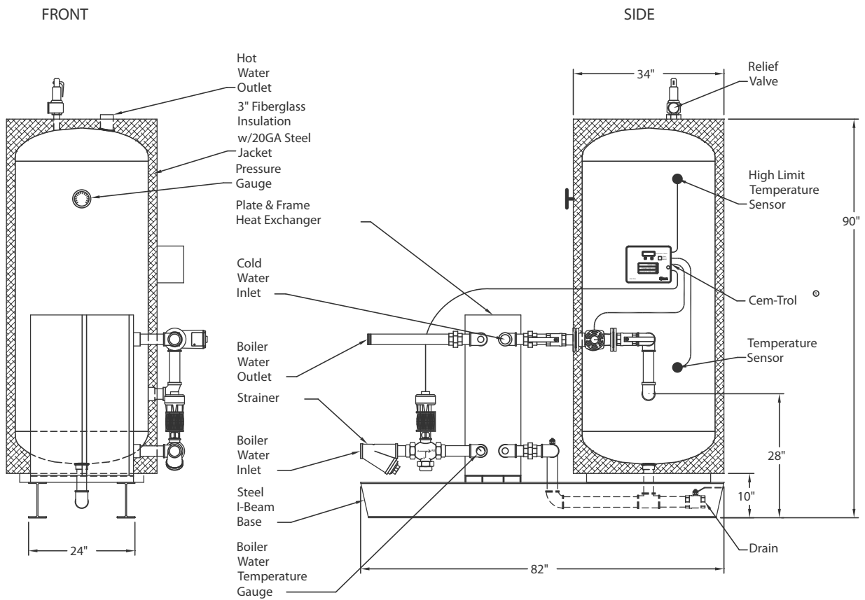
V200SPH-PF-2W PLATE & FRAME HEAT EXCHANGER
