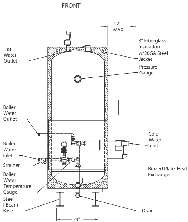
V200SPH-BP-2W BRAZED PLATE HEAT EXCHANGER
