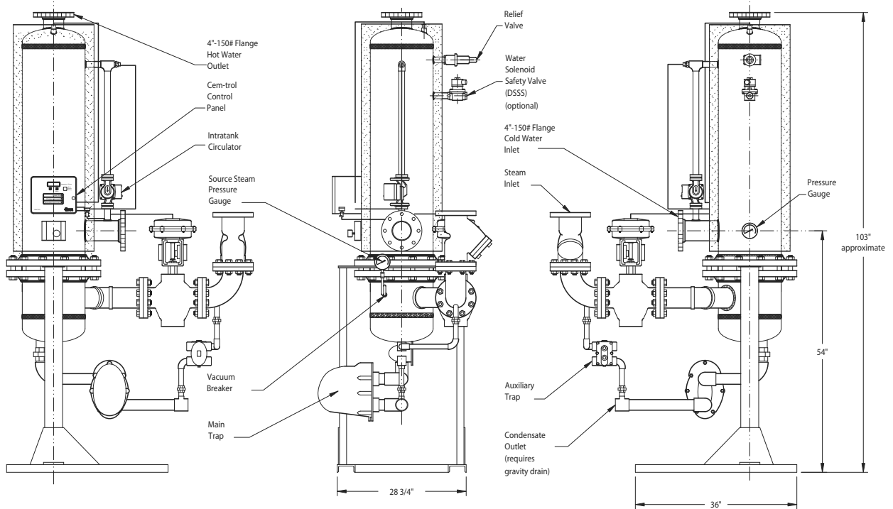
V14SEH1442 Energy Source - Steam
