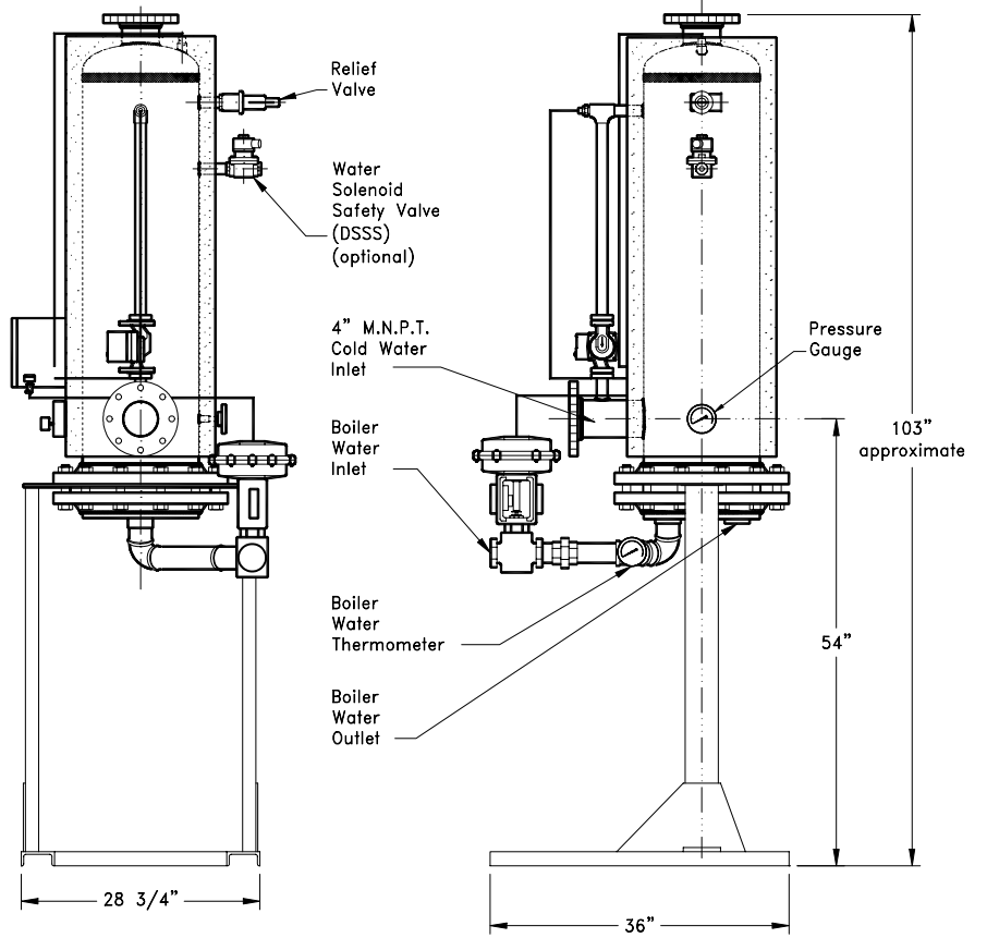
V14SEH1442 Energy Source - Boiler Water
