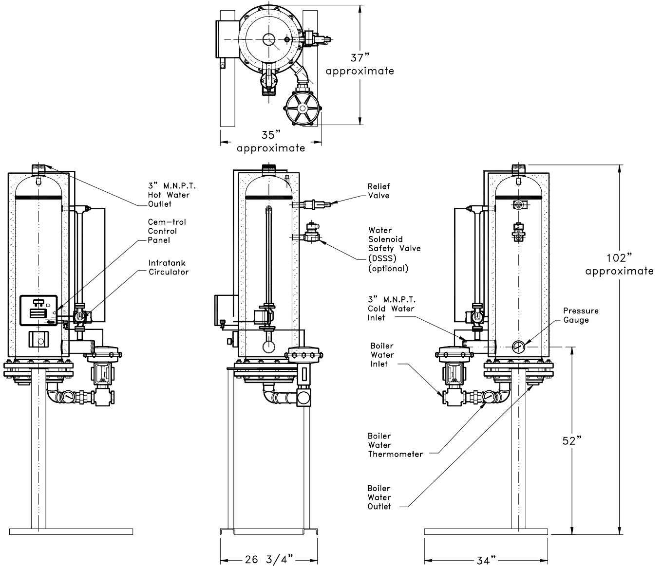
V12SEH1242 Energy Source - Boiler Water
