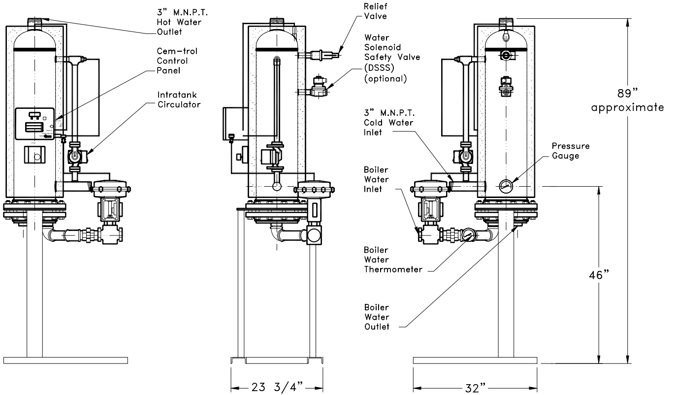
V10SEH1036 Energy source - boiler water
