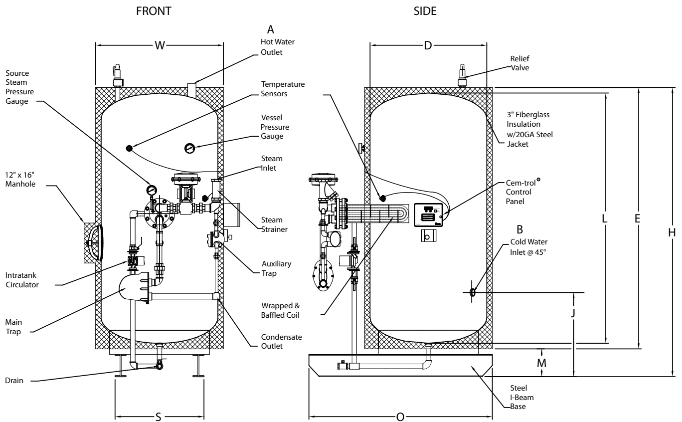
SWH-Vertical-Steam
