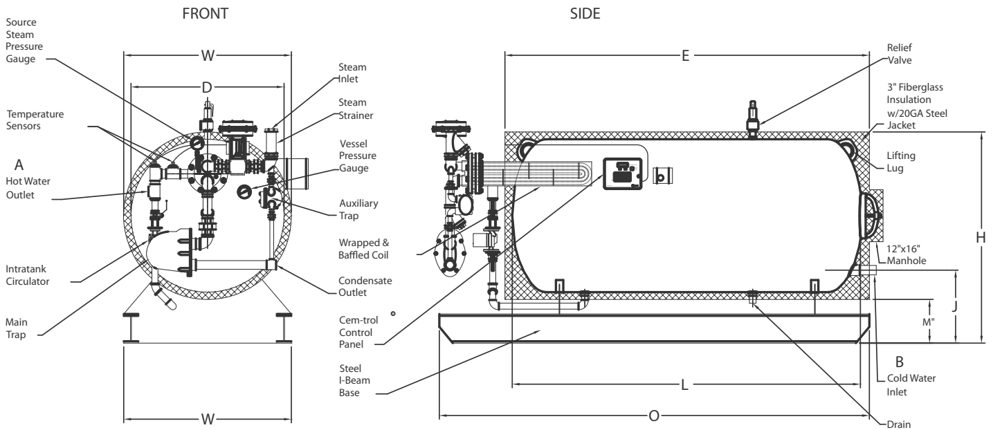
SWH-Horizontal-Steam Reverse Flow Design
