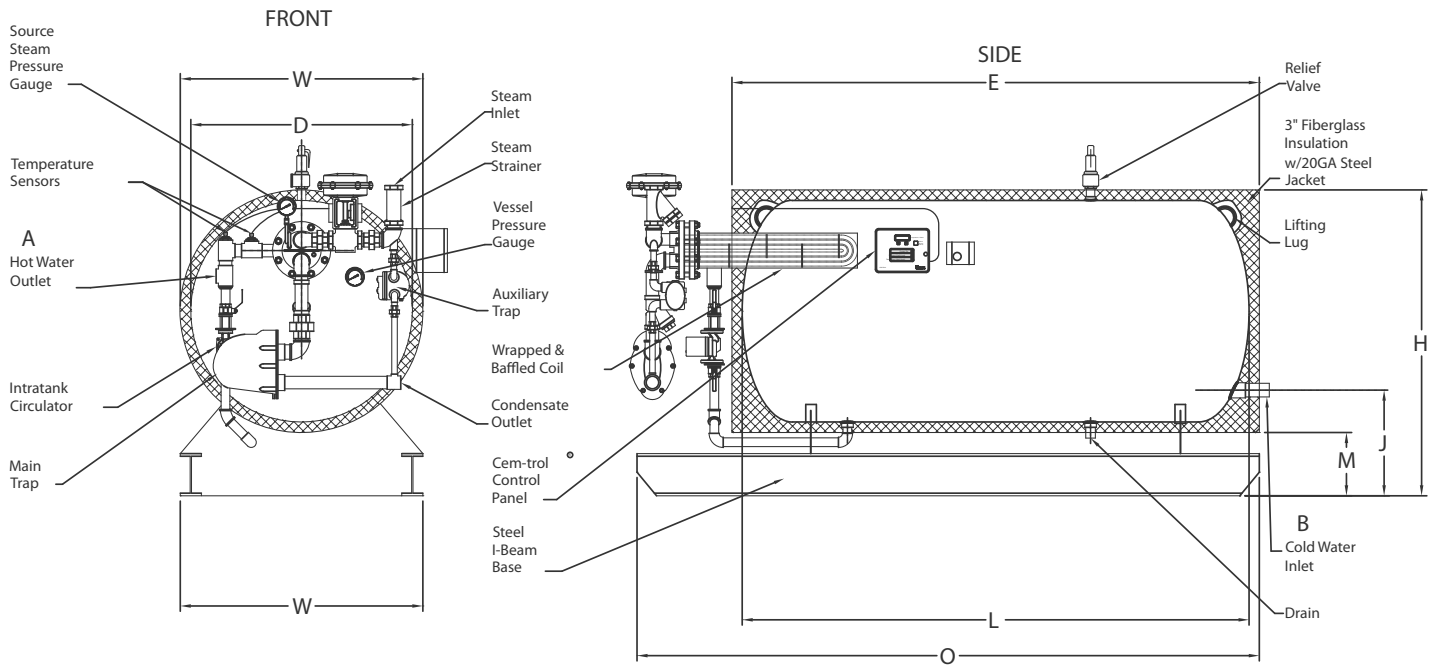
SWH-Horizontal-Steam Reverse Flow Design
