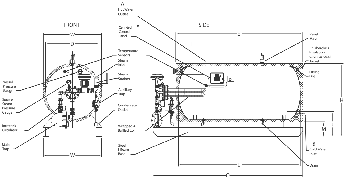
SWH-Horizontal-Steam
