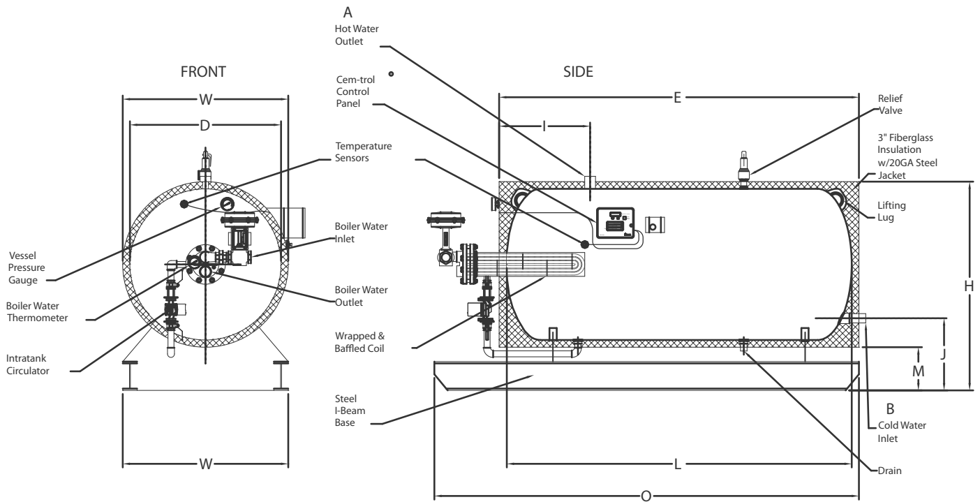
SWH-Horizontal-Boiler Water
