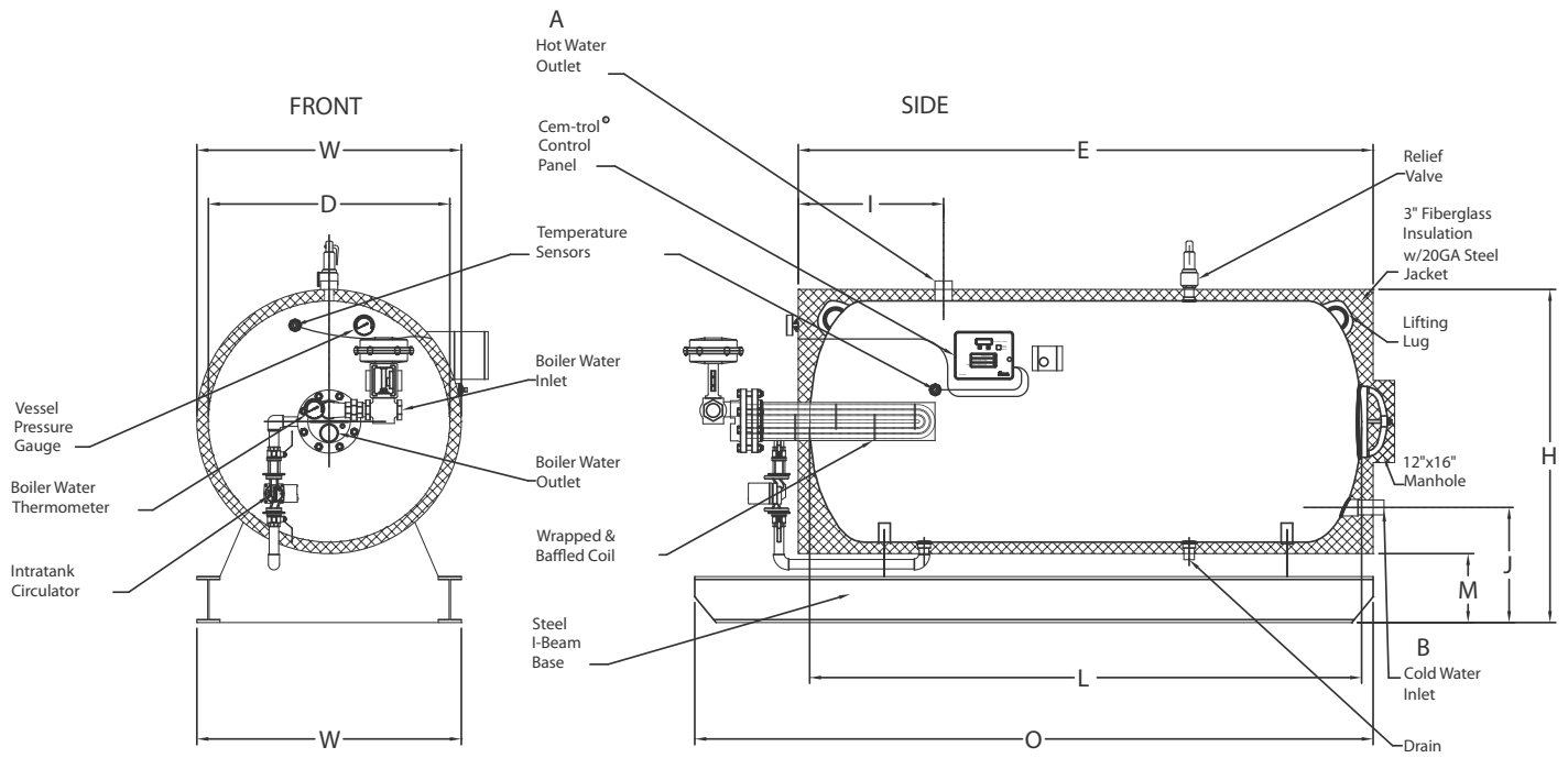
SWH-Horizontal-Boiler Water
