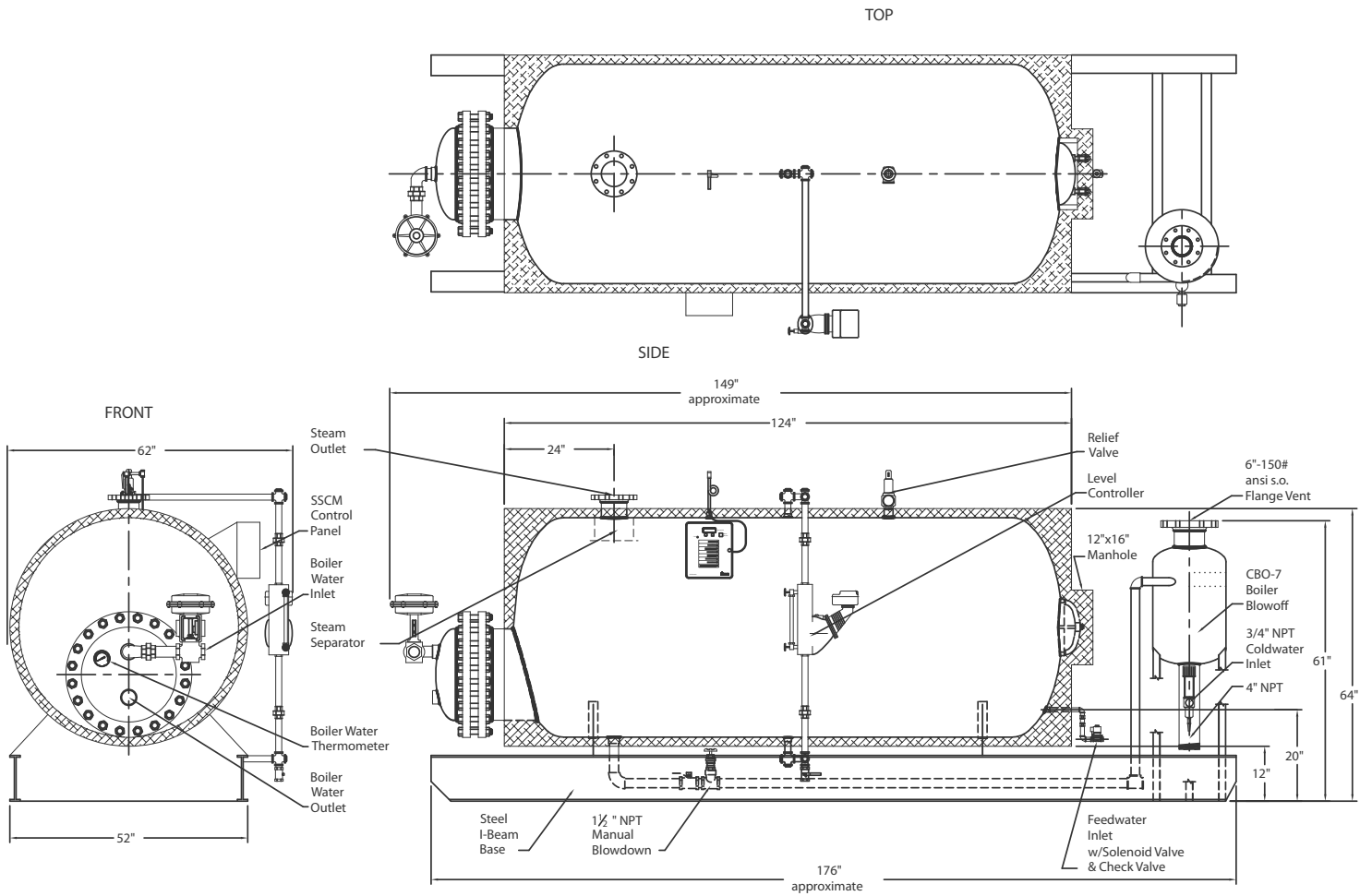
H860USG20XX-W-CBO Energy Source-Boiler Water
