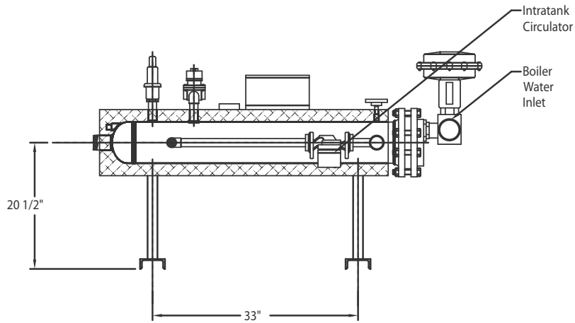
H6SEH636 Energy source - Boiler Water
