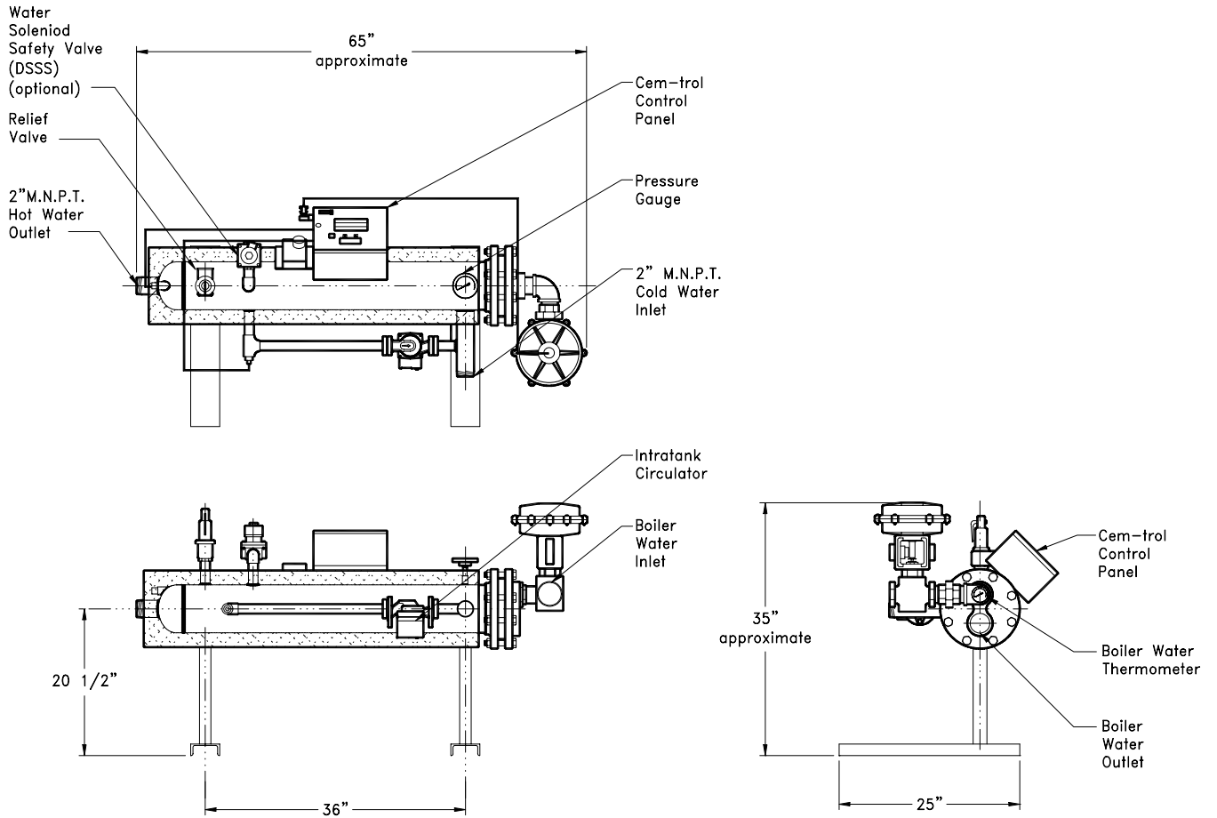
H6SEH624 Energy source – Boiler Water
