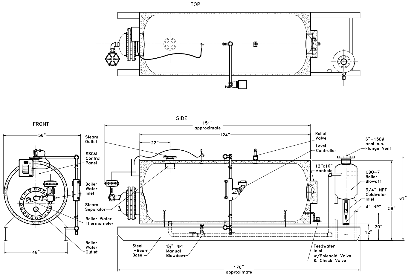
H670USG16XX-W-CBO Energy Source-Boiler Water
