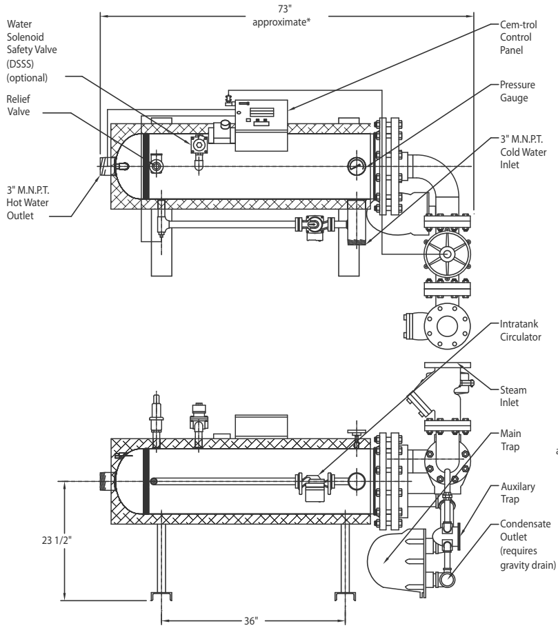
H12SEH1242 Energy source - Steam
