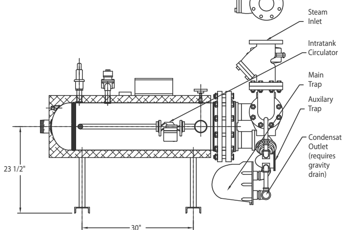
H12SEH1236 Energy source - Steam
