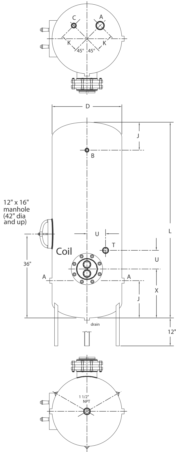
CST Vertical w/coil Angle Legs
