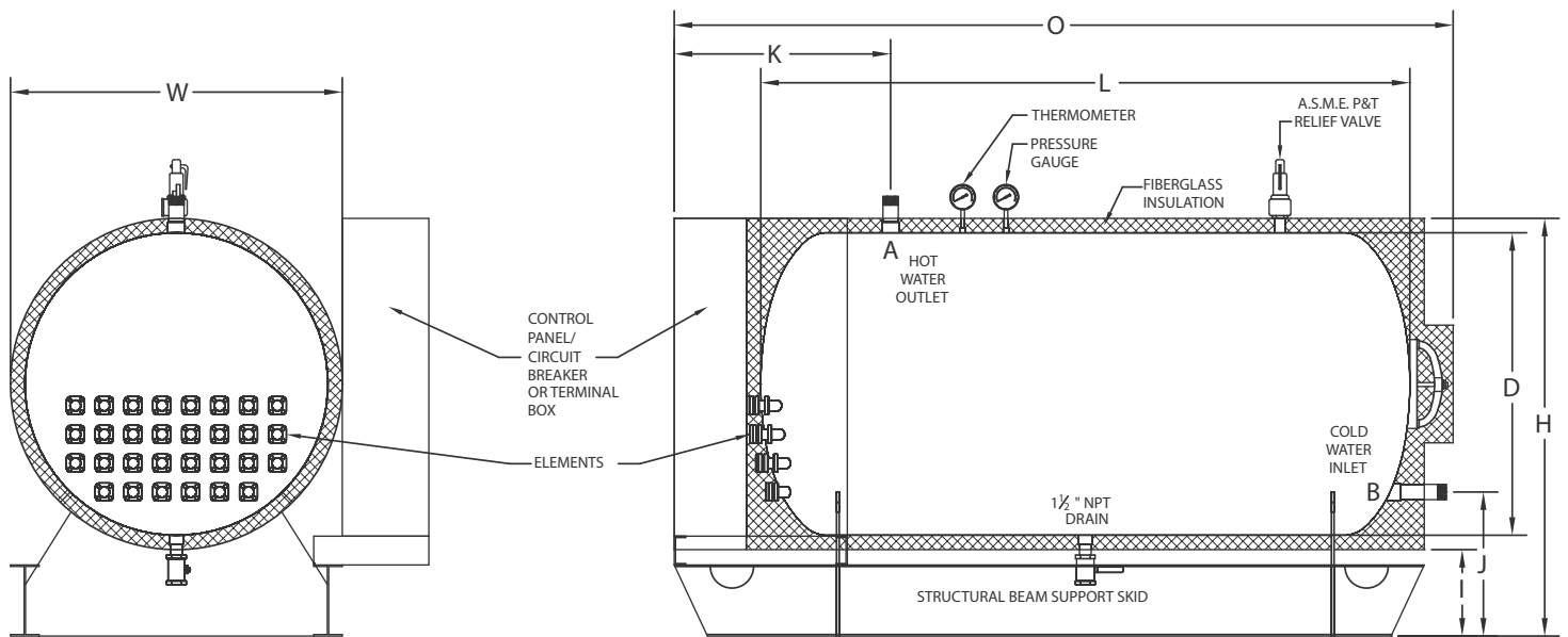
EHB - HORIZONTAL 42"+ DIAMETER (8 TO 10 STEPS)
