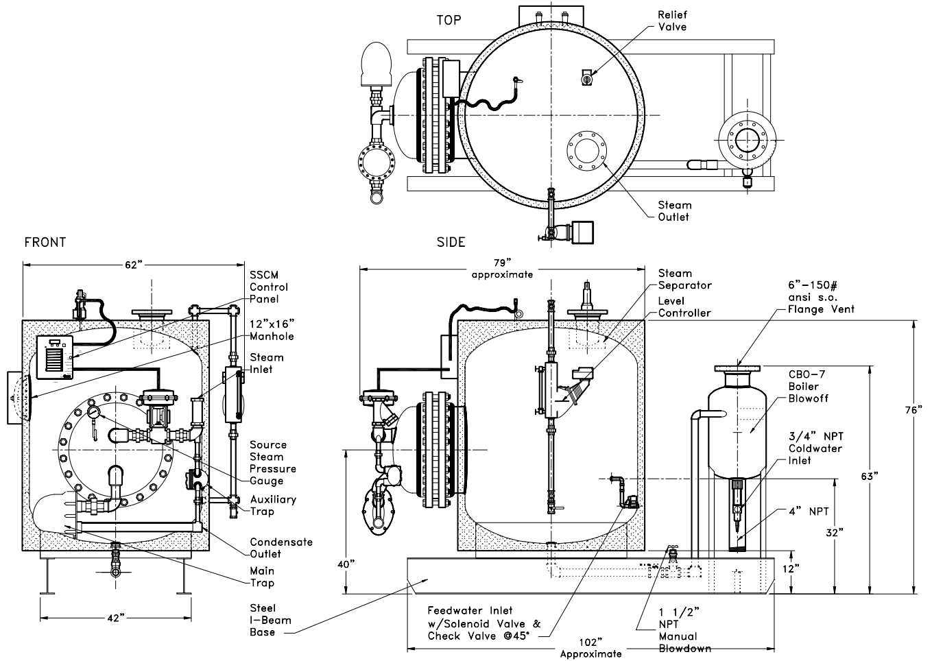
V410USG-CBO Energy Source-Steam
