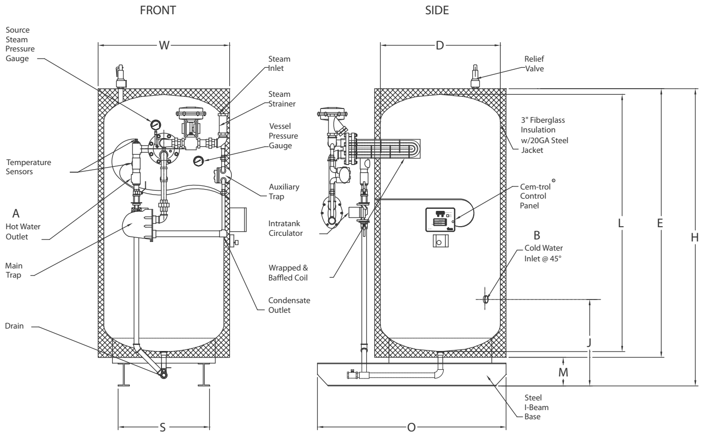
SWH-Vertical-Steam Reverse Flow Design
