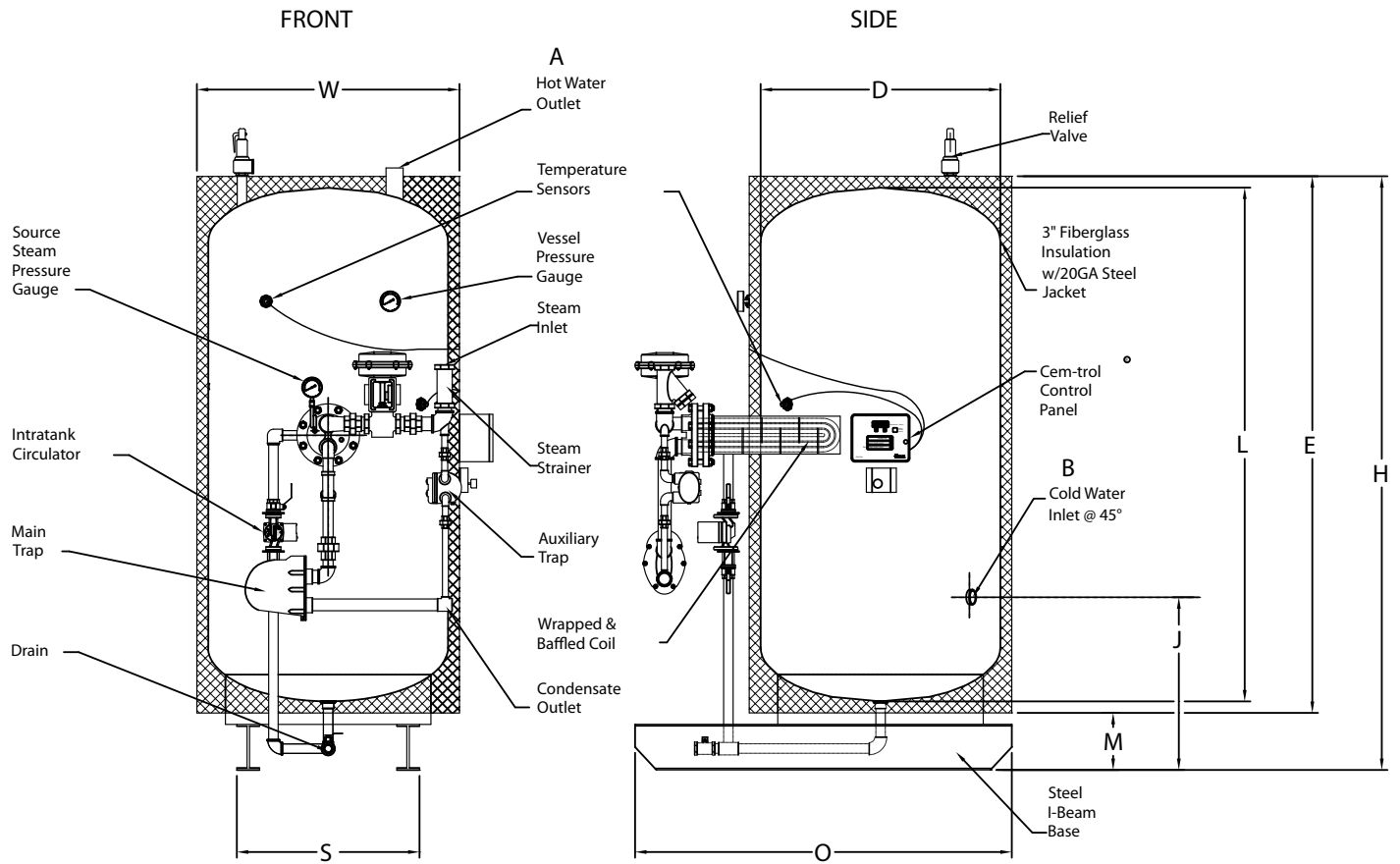
SWH-Vertical-Steam
