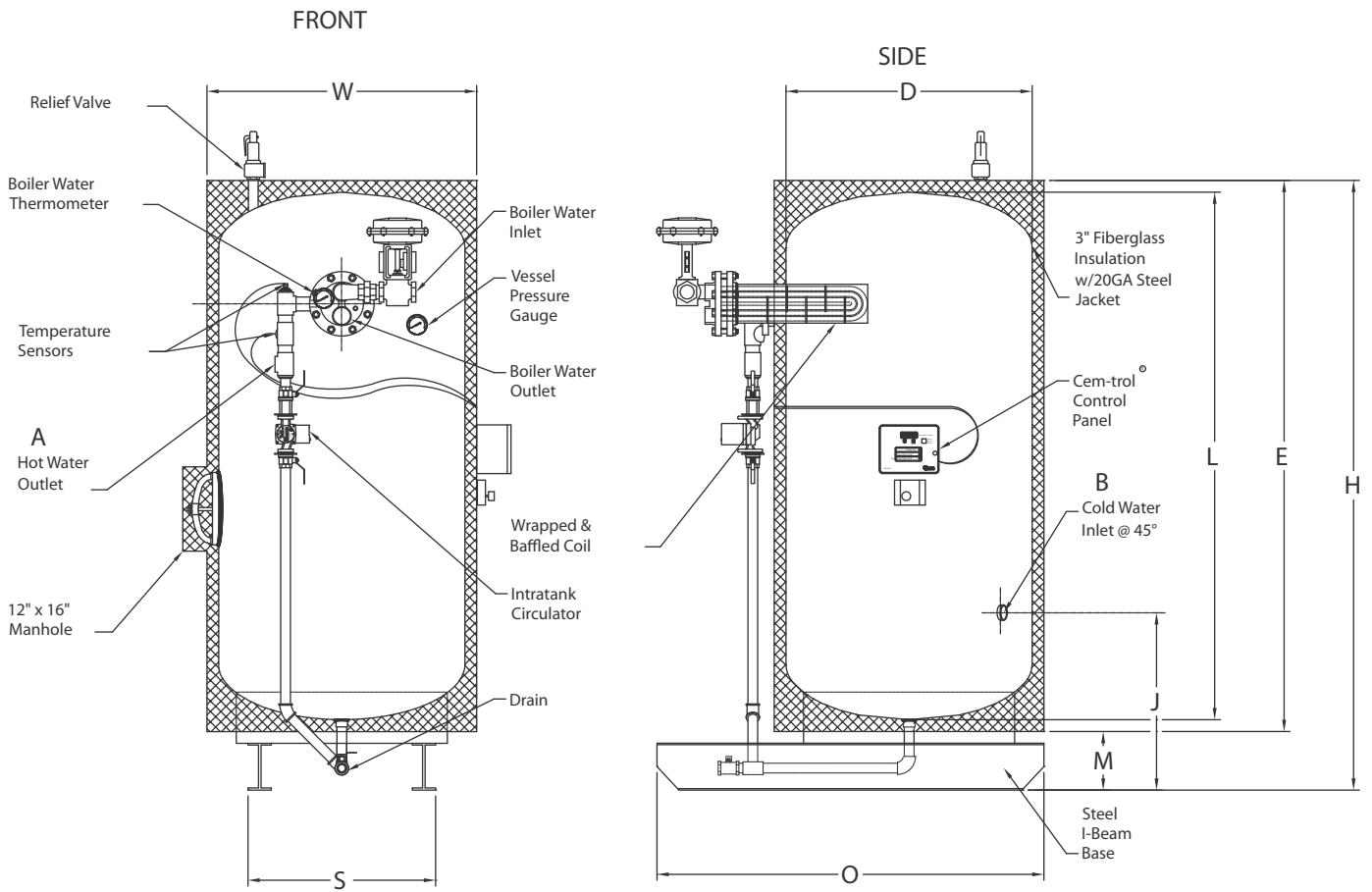
SWH-Vertical-Boiler Water Reverse Flow Design
