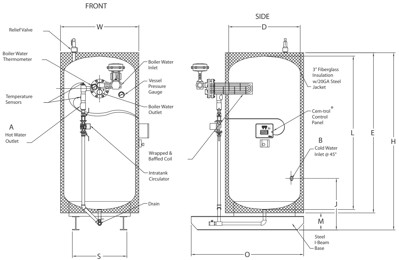
SWH-Vertical-Boiler Water Reverse Flow Design
