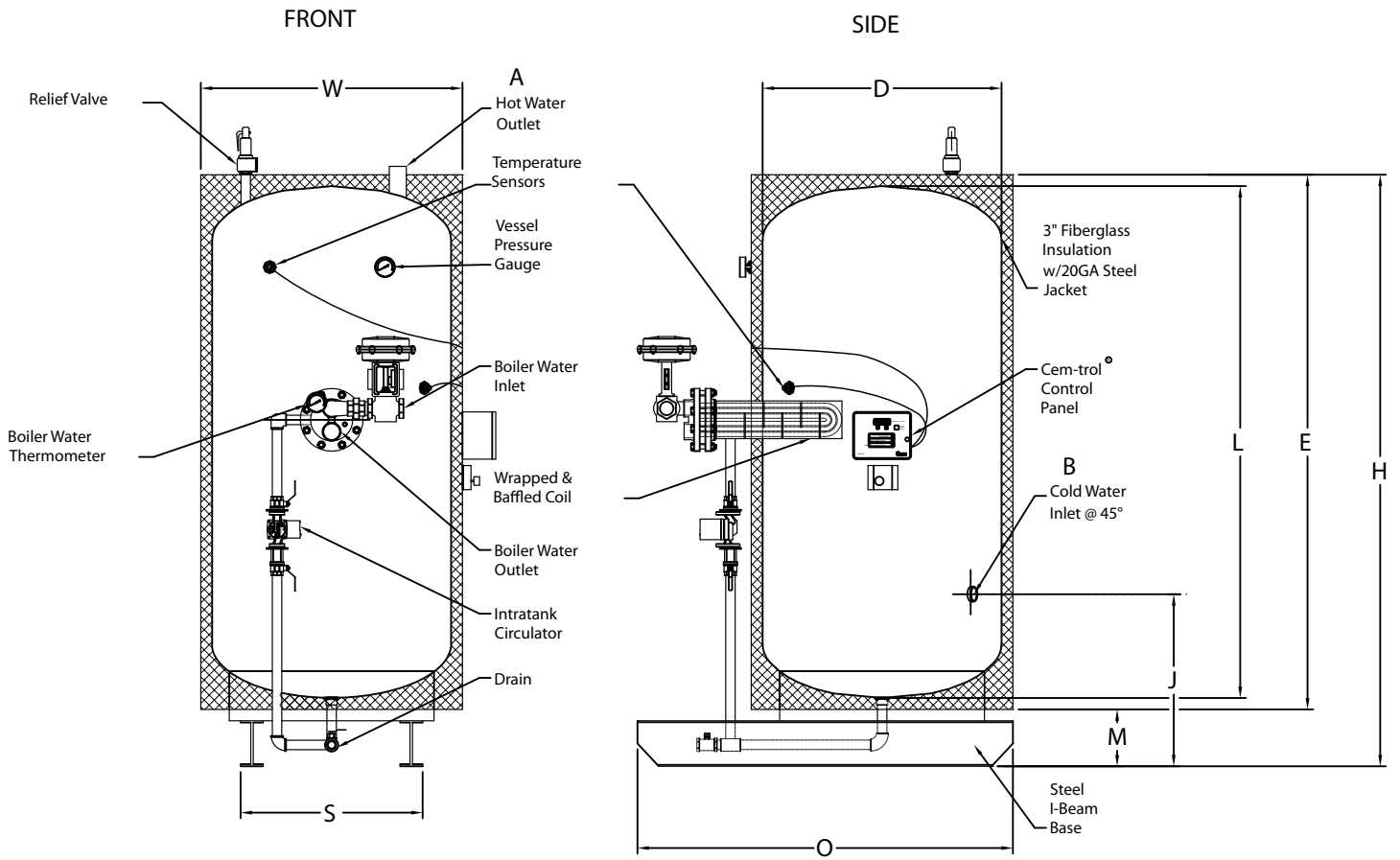
SWH-Vertical-Boiler Water
