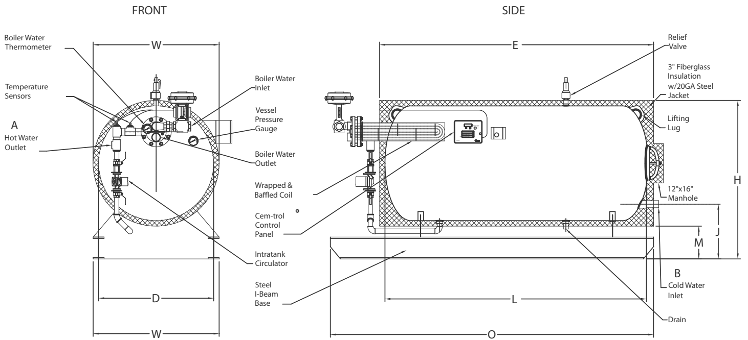
SWH-Horizontal-Boiler Water Reverse Flow Design
