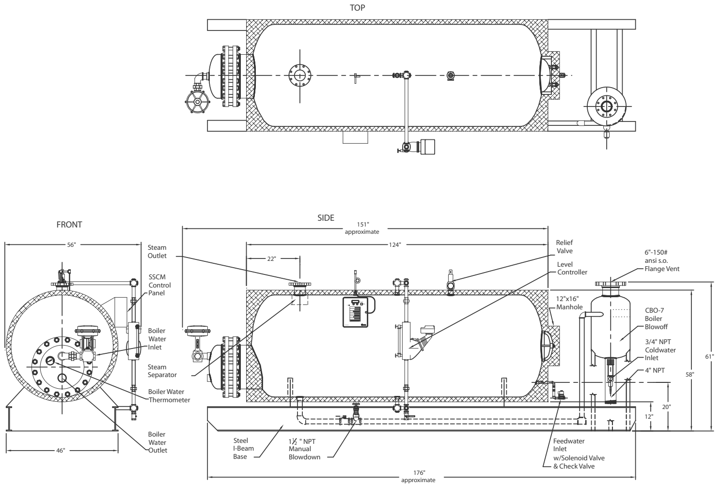
H670USG18XX-W-CBO Energy Source-Boiler Water
