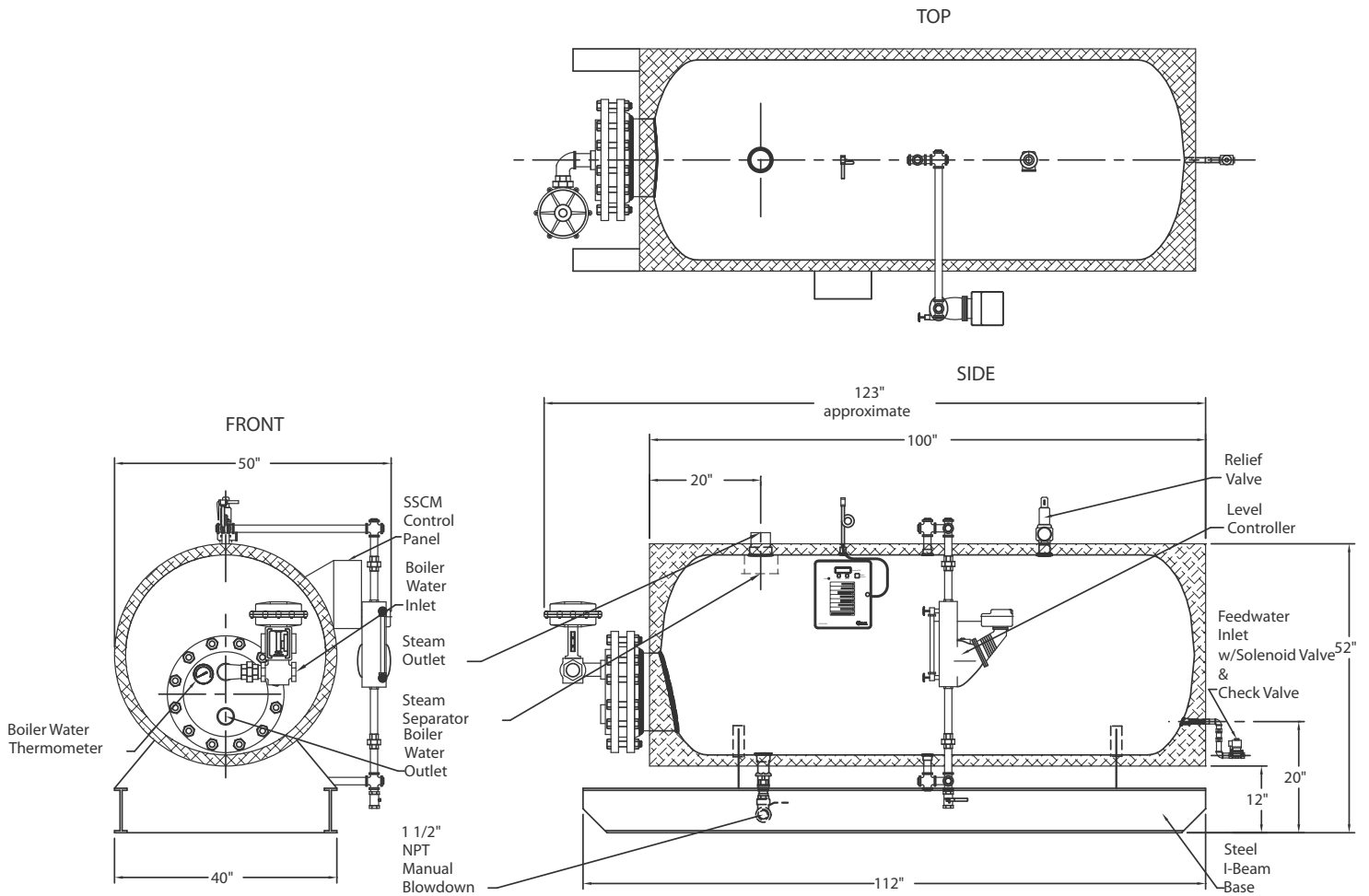
H395USG14xx-W Energy Source-Boiler Water
