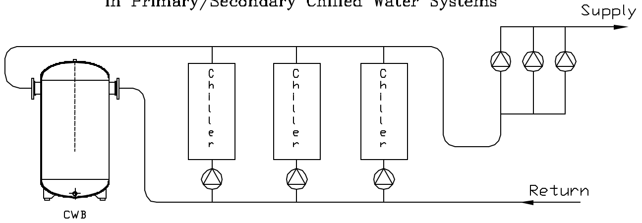
Back Loaded Common & Storage Tank
