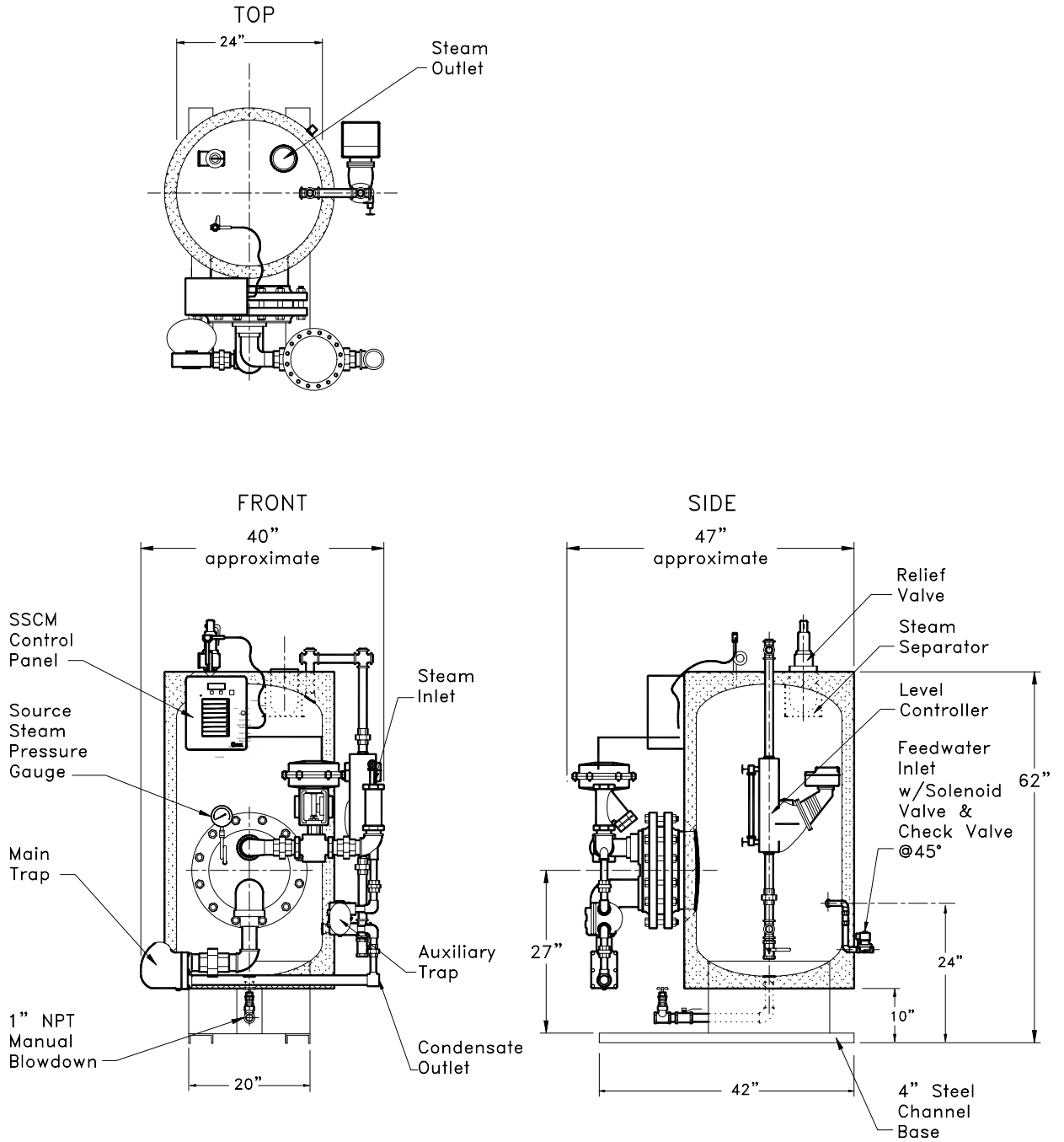
V90USG Energy Source - Steam
