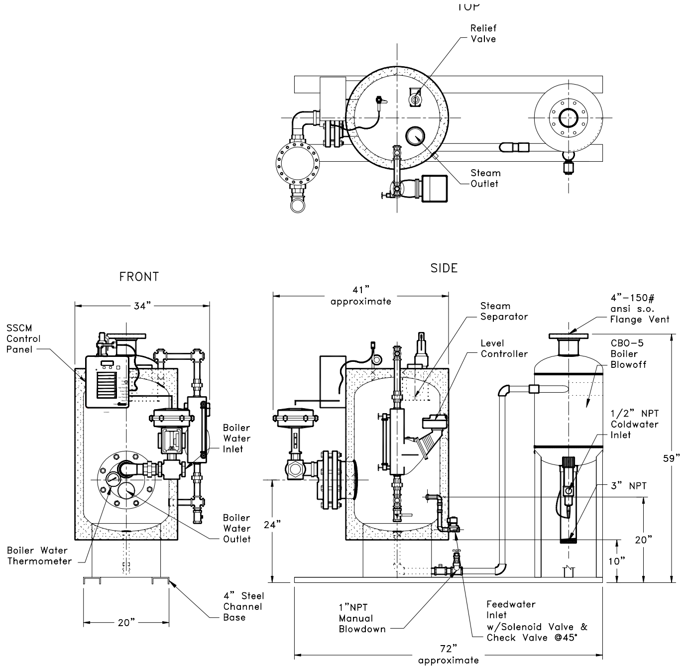
V45USG-W-CBO Energy Source - Boiler Water
