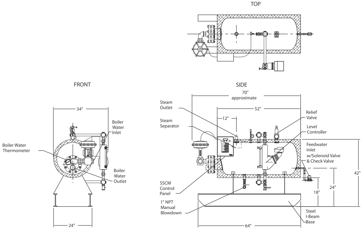
H60USG6XX-W Energy Source-Boiler Water
