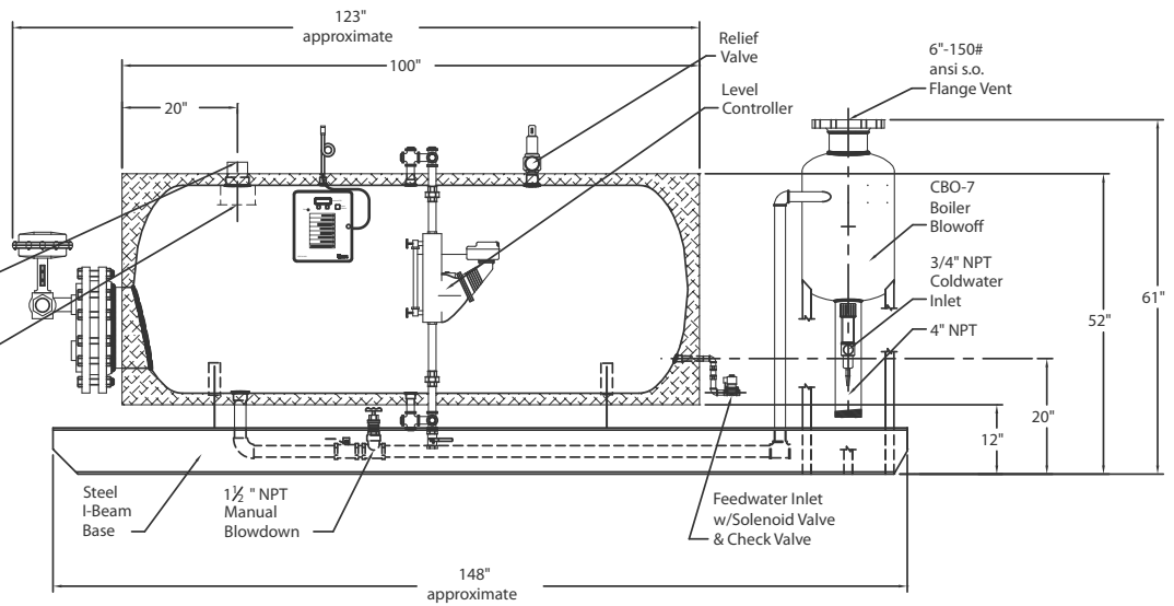
SIDE
