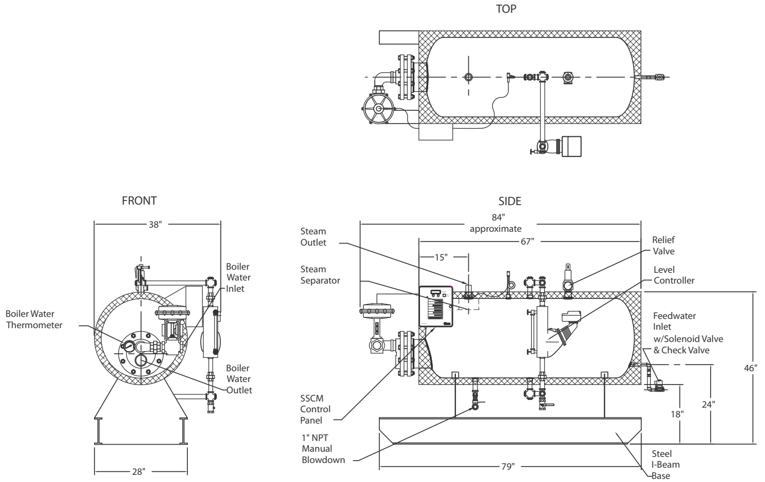
H120USG8XX-W Energy Source-Boiler Water
