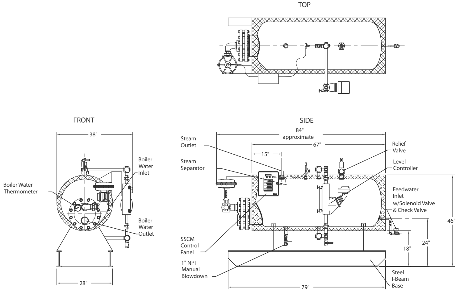
H120USG10XX-W Energy Source-Boiler Water
